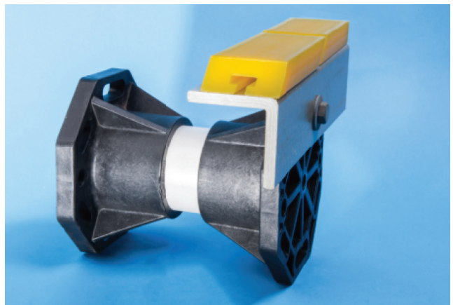
FRP ANGLE WITH UHMW WEAR STRIP
