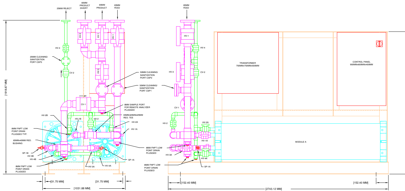
CATHODE END VIEW
