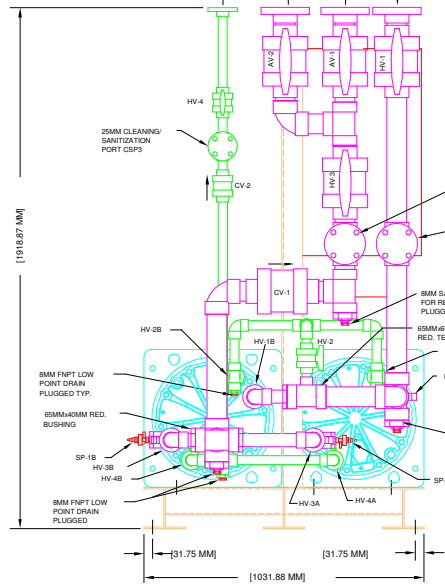
CATHODE END VIEW
